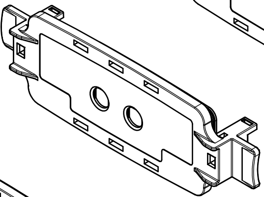
CABLE GLAND LATCH FACEPLATE ECS-P-122X169-L-UV1-CG ECS-P-122X169-L-UV-CG GY
