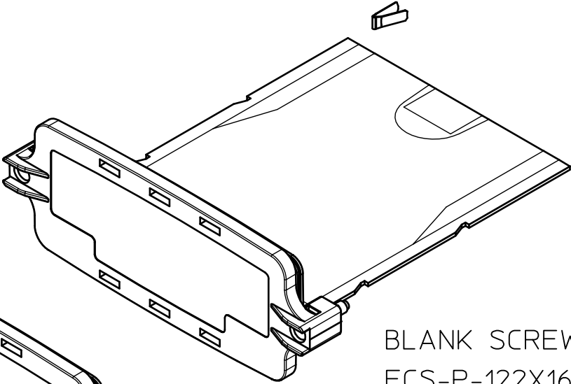
1-M12 SCREW FACEPLATE ECS-P-122X169-S-UV1-1M12 ECS-P-122X169-S-UV-1M12 GY
