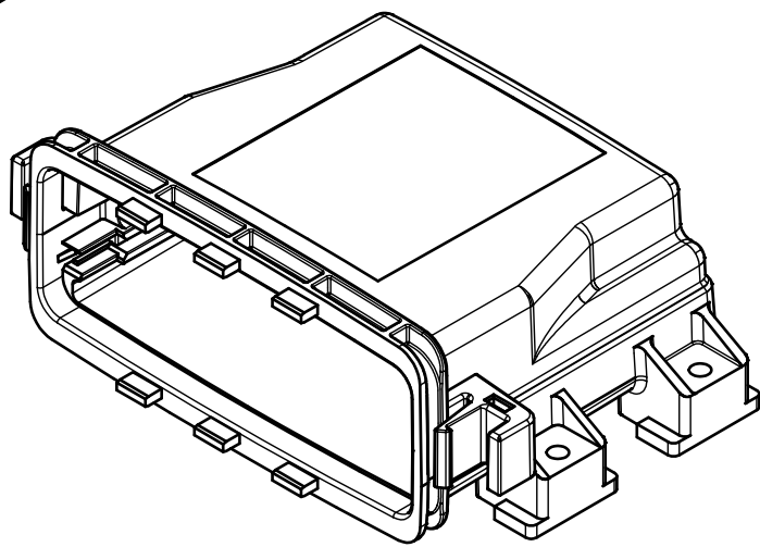
NON VENTED LATCH ENCLOSURE 122X169 ECS-B-122X169-L-UV1-NV ECS-B-122X169-L-UV-NV GY
