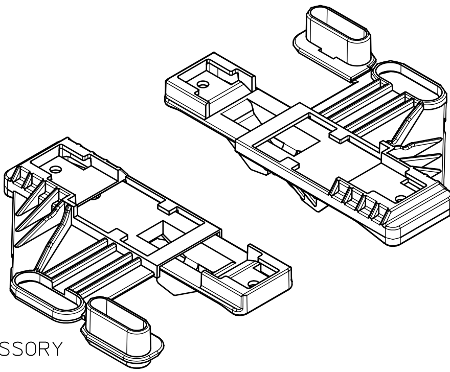
BOARD LOCK ACCESSORY ECS-BL
