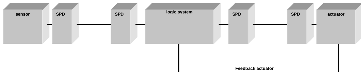
Figure 29: Connection for fault detection
