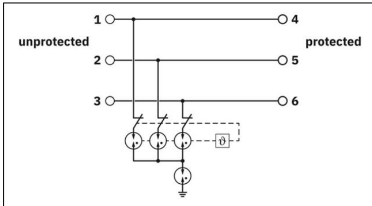
Figure 25: Circuit diagram of TTC-6P-3-APL-(EX-)24DC-UT-I
