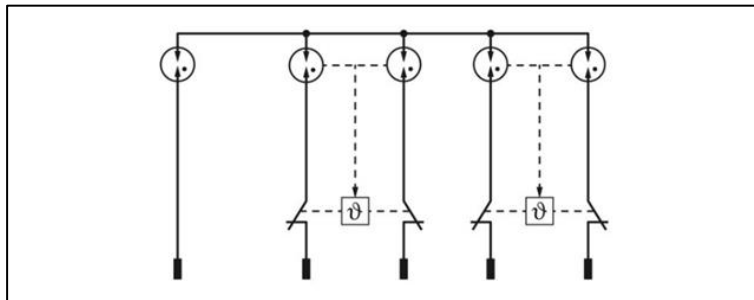
Figure 26: Circuit diagram of TTC-6P-4-GDT-(EX-)24DC-I-P
