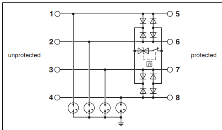
Figure 24: Circuit diagram of TTC-6P-4-...DC-...-I
