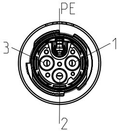
plug face male
