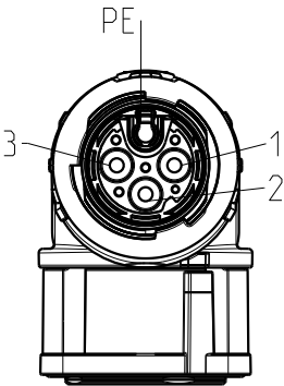
plug face male
