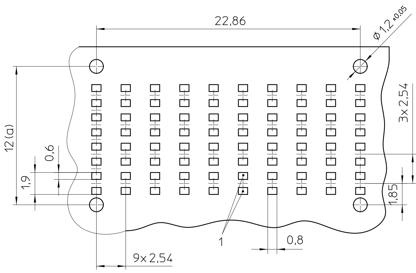
recommended PCB layout view: component side
