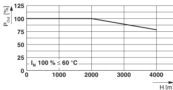
Figure 20 Output power depending on the installation height
