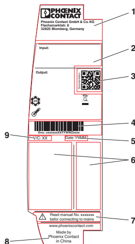
Figure 2 Rating plate information
