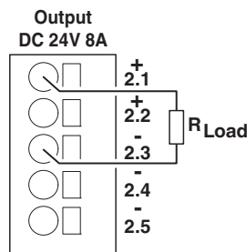
Figure 15 Schematic diagram, switching the output terminals
