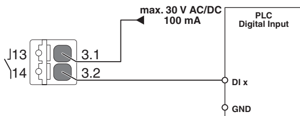
Figure 18 Wiring principle
