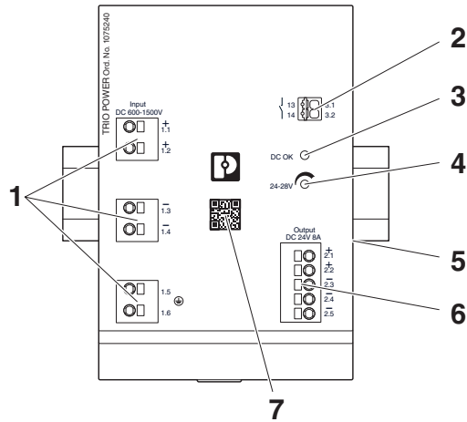
Figure 4 Function elements
