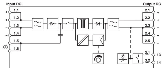
Figure 3 Block diagram
