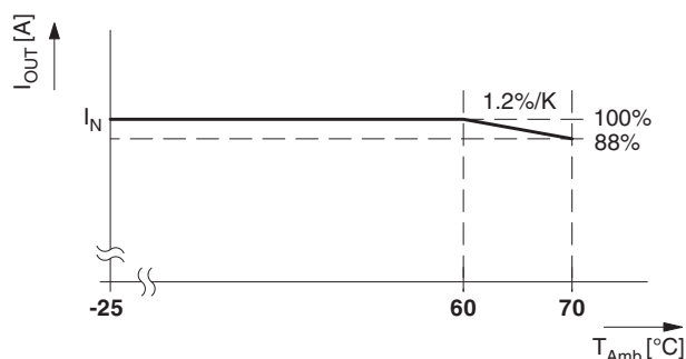
Figure 19 Temperature derating in normal mounting position
