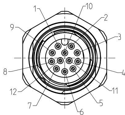
View of pin assignment Plug-in side
