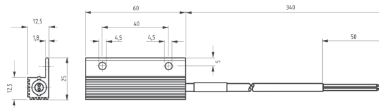
Art. No. 01610.0-00
