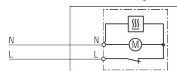
Connection diagram
