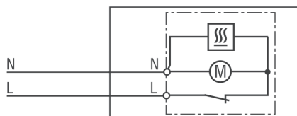
Connection diagram
