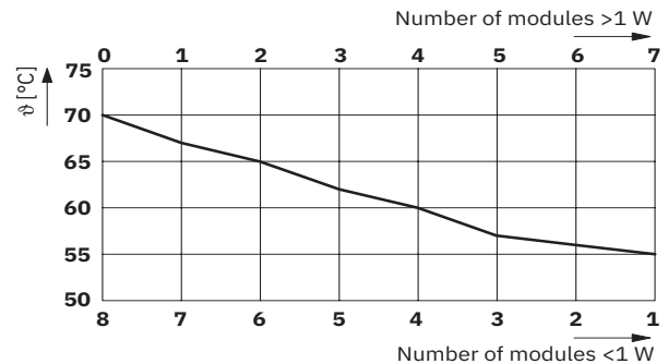
Figure 3 Derating curve
