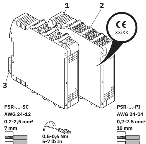
Figure 16 Connection versions
