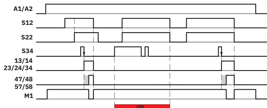
Figure 4 Time diagram for on delay, manual start
