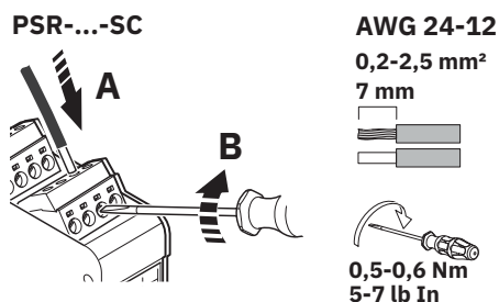
Figure 20 Connecting the cables for PSR-...-SC (screw terminal block)
