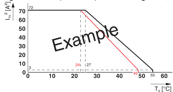
Figure 29 Example of a suspended derating curve (red)
