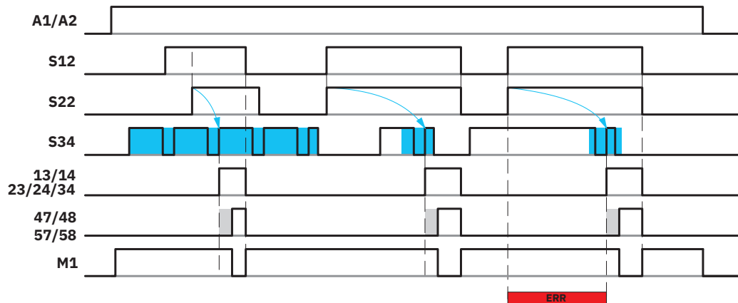
Figure 3 Time diagram for on delay, automatic start
