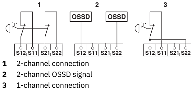
Figure 22 Signal generator connection versions
