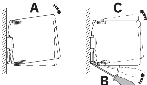
Figure 19 Mounting and removing
