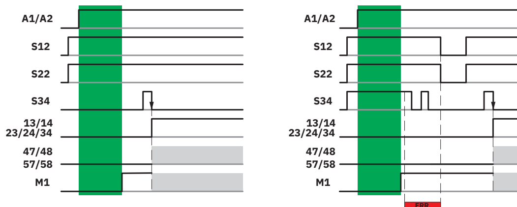
Figure 2 Time diagram for power-up, manual start
