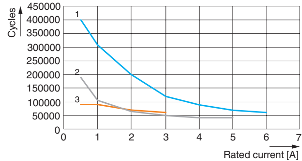
Figure 15 Electrical service life
