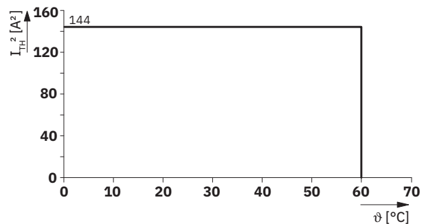
Figure 13 Derating curve - horizontal mounting position with 10 mm spacing
