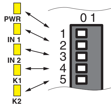
Figure 25 Assignment of LEDs and DIP switch poles
