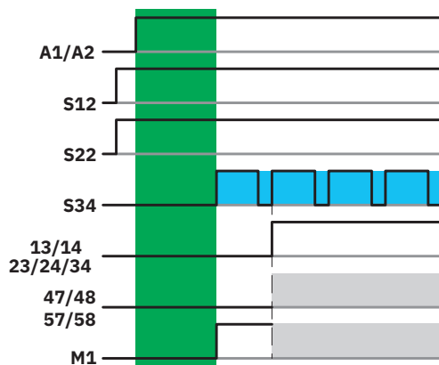
Figure 1 Time diagram for power-up, automatic start
