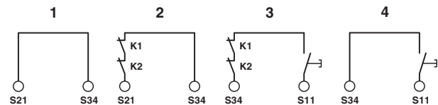
Figure 23 Start and feedback circuit connection variants
