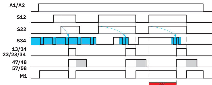
Figure 6 Time diagram for off delay, automatic start
