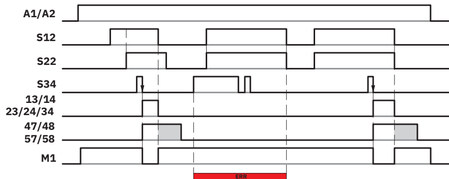
Figure 7 Time diagram for off delay, manual start
