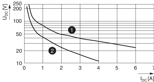
Figure 14 Load limit curve - ohmic and inductive load
