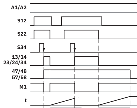
Figure 9 Time diagram for off delay, manual start, can be re-triggered
