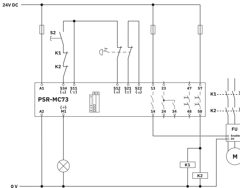
Figure 27 Emergency stop monitoring/manual, monitored start
