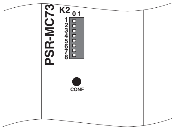
Figure 24 CONF button and DIP switch
