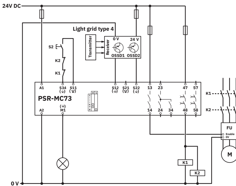
Figure 28 Light grid monitoring/manual, monitored start
