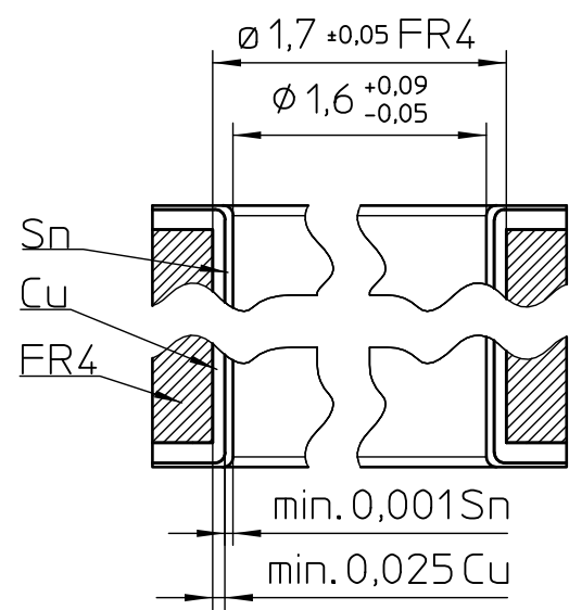
plated hole configuration 50:1
