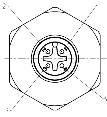
View of pin assignment Plug-in side
