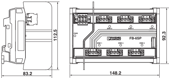
Figure 1 FB-6SP
