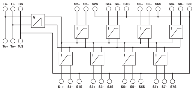
Figure 4 FB-8SP circuit diagram
