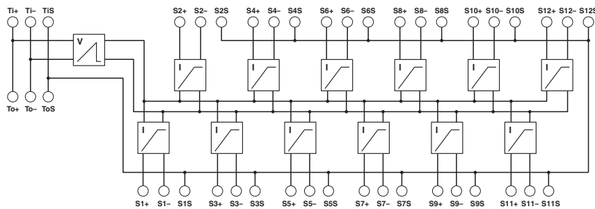
Figure 5 FB-12SP circuit diagram
