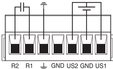
Figure 4 Single power supply connection
