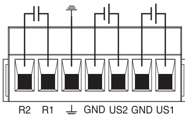
Figure 3 Redundant power supply connection
