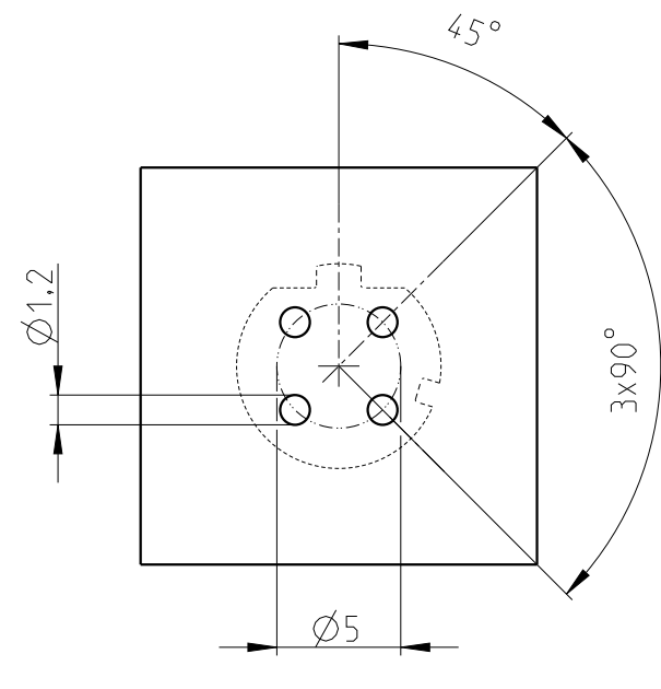
PCB-layout (advice)
