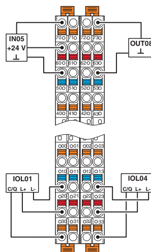
Figure 3 Connection example
