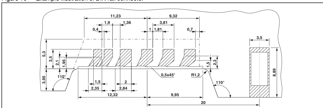
Figure 10 Example illustration of DIN rail connector
