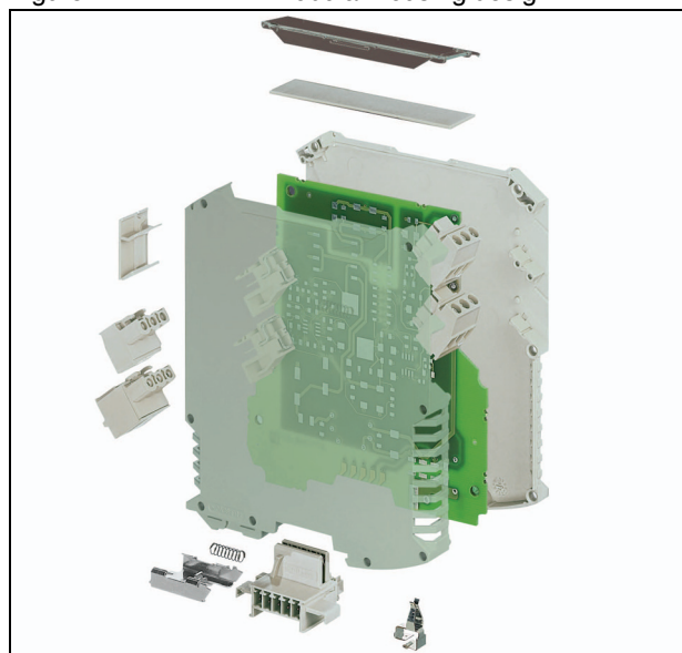
Figure 1 ME MAX modular housing design
