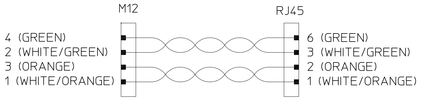
WIRING DIAGRAM
