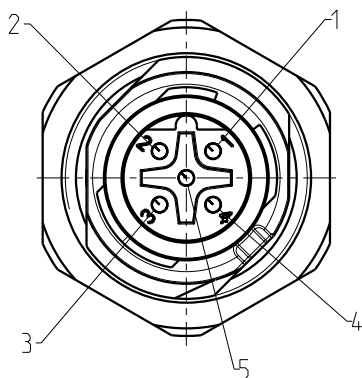
View of pin assignment Plug-in side
