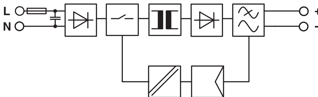
Block diagram
